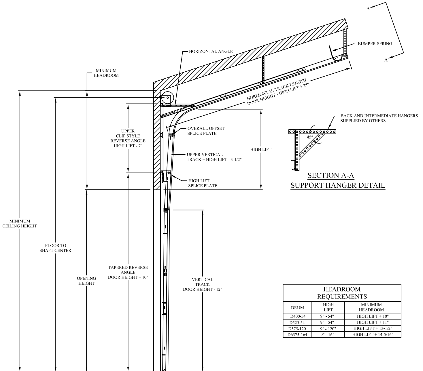
HIGH LIFT TAPERED REVERSE ANGLE MOUNT TRACK SET DETAIL
